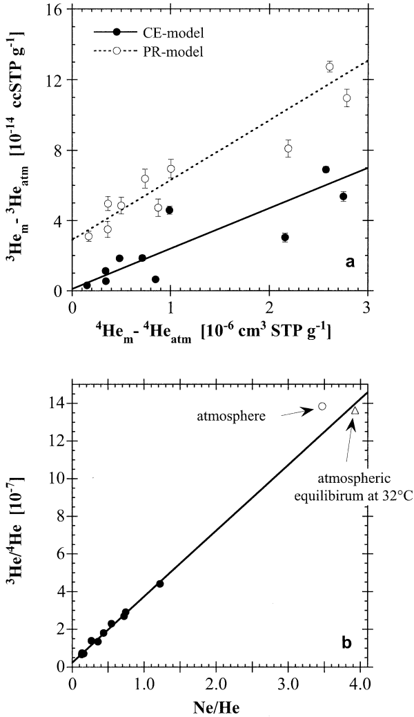
Fig. 6. Different methods to estimate (^3\text{He}/^4\text{He})_{\text{ter}} . (a) Non-atmospheric ^3\text{He} versus non-atmospheric ^4\text{He} for intermediate and old groundwater samples ( \text{He}_{\text{ter}} > 1.5 \cdot 10^{-7} \text{ cm}^3 \text{STP g}^{-1} ) from the CT aquifers. Assuming a constant prebomb tritium and a constant (^3\text{He}/^4\text{He})_{\text{ter}} the intercept of the regression line corresponds to ^3\text{He}_{\text{tri}} and the slope corresponds to (^3\text{He}/^4\text{He})_{\text{ter}} . Based on the concentrations of Ne, Ar, Kr, and Xe, ^3\text{He}_m - ^3\text{He}_{\text{atm}} and ^4\text{He}_m - ^4\text{He}_{\text{atm}} are determined using the PR-model (open circles) and the CE-model (solid circles), respectively. (b) Measured ^3\text{He}/^4\text{He} ratio versus the measured concentration ratio of Ne to He. If the He concentration approaches infinity, the Ne/He ratio approaches zero and the atmospheric gas contribution becomes negligible compared to terrigenous contributions. Thus the intercept of the regression line in Fig. 5b can be interpreted to correspond to (^3\text{He}/^4\text{He})_{\text{ter}} .
